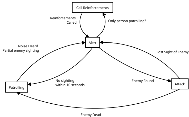
Figure 339: Finite state machine representing an enemy AI
